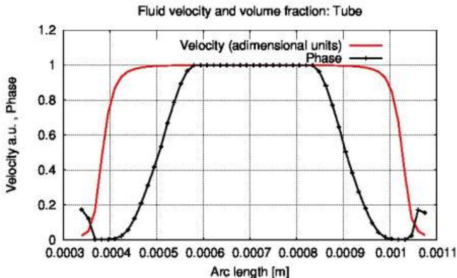
Figure 7 Fluid solution: velocity and volume fraction profiles along a section of the focusing tube.
