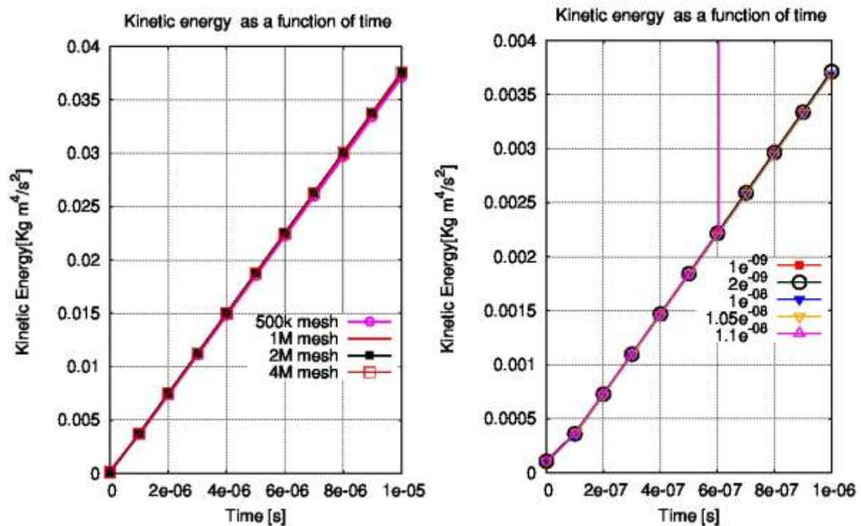
Figure 4 Dependency of the Kinetic energy from the grid and time step resolution.
