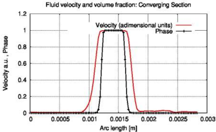
Figure 6 Fluid solution: velocity and volume fraction profiles along the converging nozzle section.
