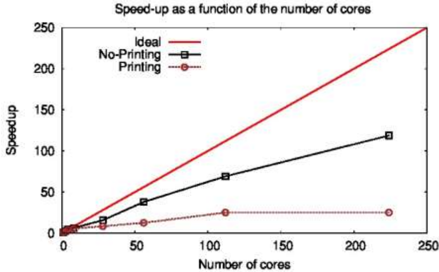
Figure 9 Speedup as a function of number of cores with a printing rate of 1/100 step (Printing) and 1/1000 step (No-printing)
