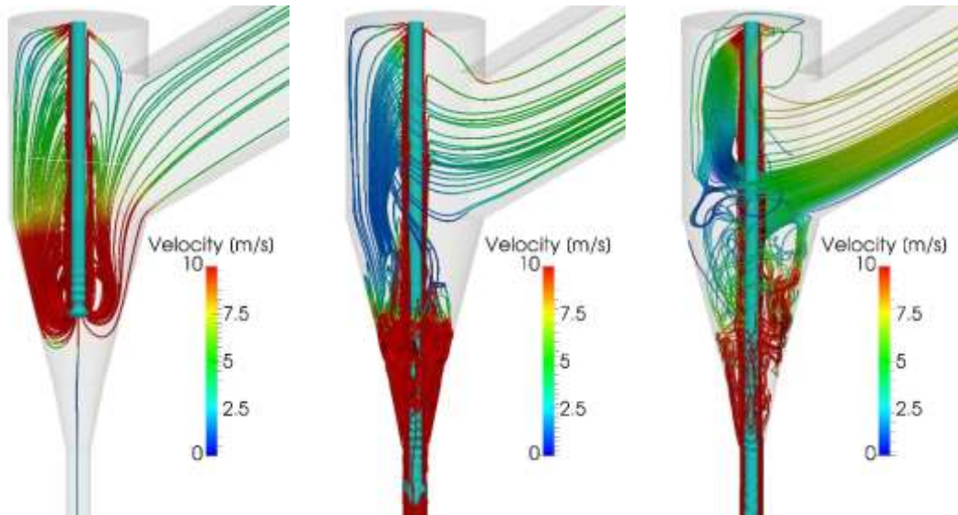
Figure 2 Characteristic moment on the jet formation. Jet forming in the mixing chamber (left), Jet entering the tubular part (center), and fully developed jet (Right). The jet is colored in blue, streamlines of the velocity field are present
