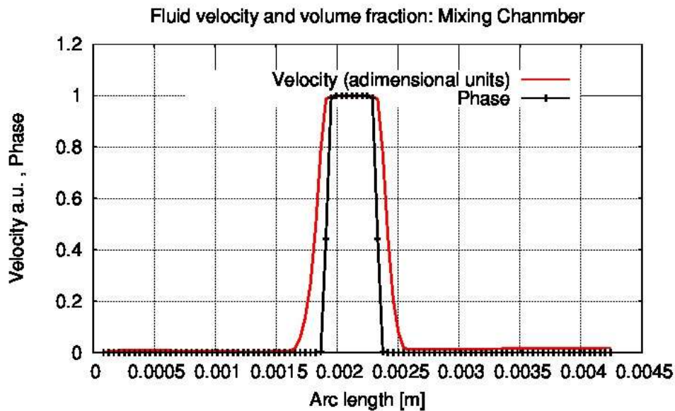
Figure 5 Stabilized jet: velocity and volume fraction profiles in the mixing chamber
