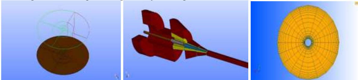
Figure 1 Structured mesh generation with Salome: Single block definition (Left), Block assembly (center) and mesh refinements (right)
