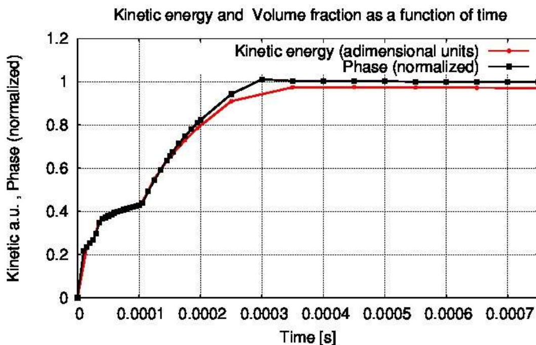
Figure 3 Kinetic energy and volume fraction as functions of time during the simulation. During the Jet development, the kinetic energy of the system increases, until reaching a stable value when the jet stabilizes.
