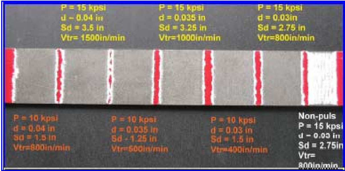
Fig. 5. Photograph showing the removal of two layers of epoxy coating from a marine steel panel with a single-orifice non-rotating FPWJ at operating conditions as indicated
