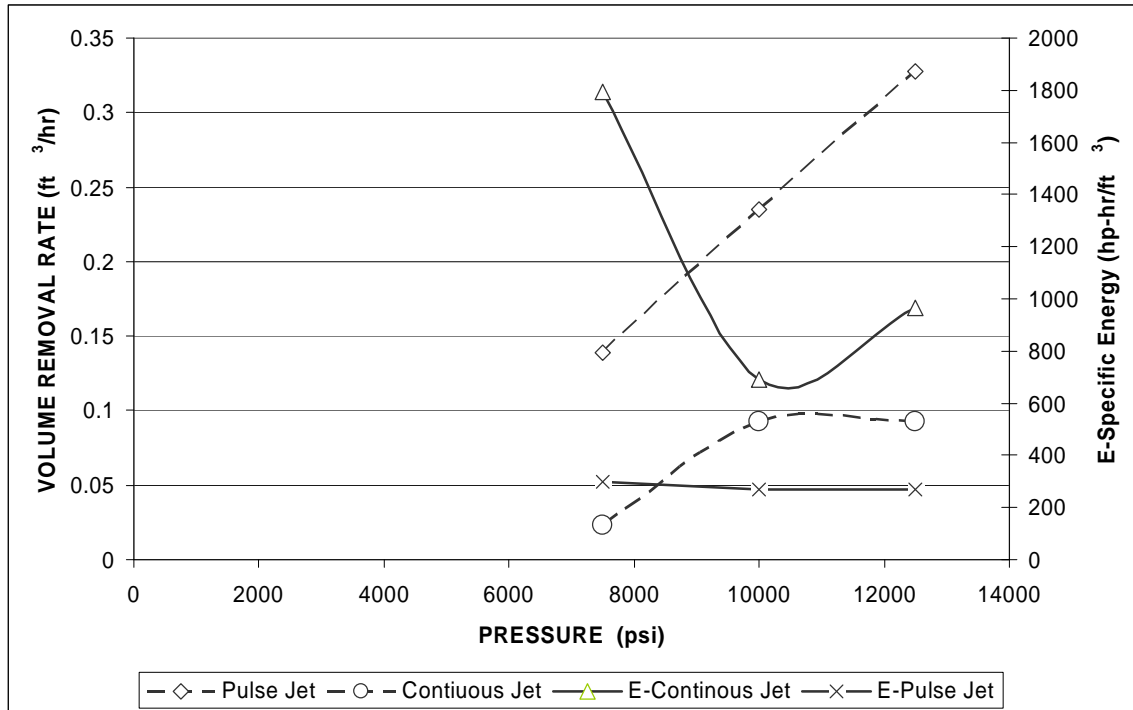
Fig. 3. Comparison of the performance of FPWJ with corresponding continuous waterjet (CWJ) for cutting granite. The data show the effect of pressure on volume removal rate and specific energy.
