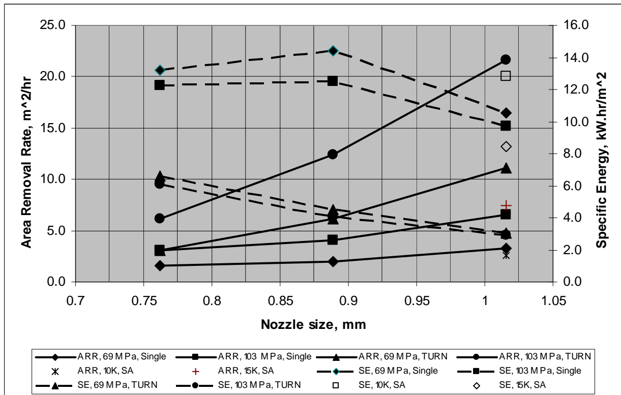
Fig. 9. Plot of removal rates and specific energies obtained with single-orifice, dual-orifice rotating (indicated by 'SA') and the TURN at the operating conditions as indicated.
