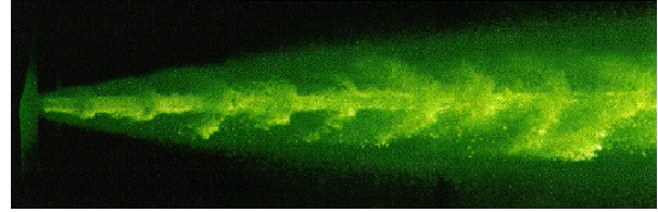
Fig. 1B. Photograph of the well-defined and fully developed FPWJ taken with a Nd-Yag Laser [6].
