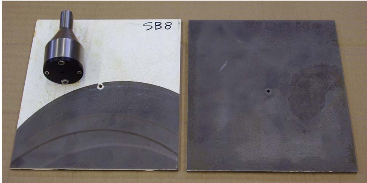
Fig. 8. Typical appearance of the substrate from which two layers of epoxy coatings were removed with the TURN (sample received from ATK Thiokol, USA). Dual-orifice rotating nozzle is shown for comparison.
