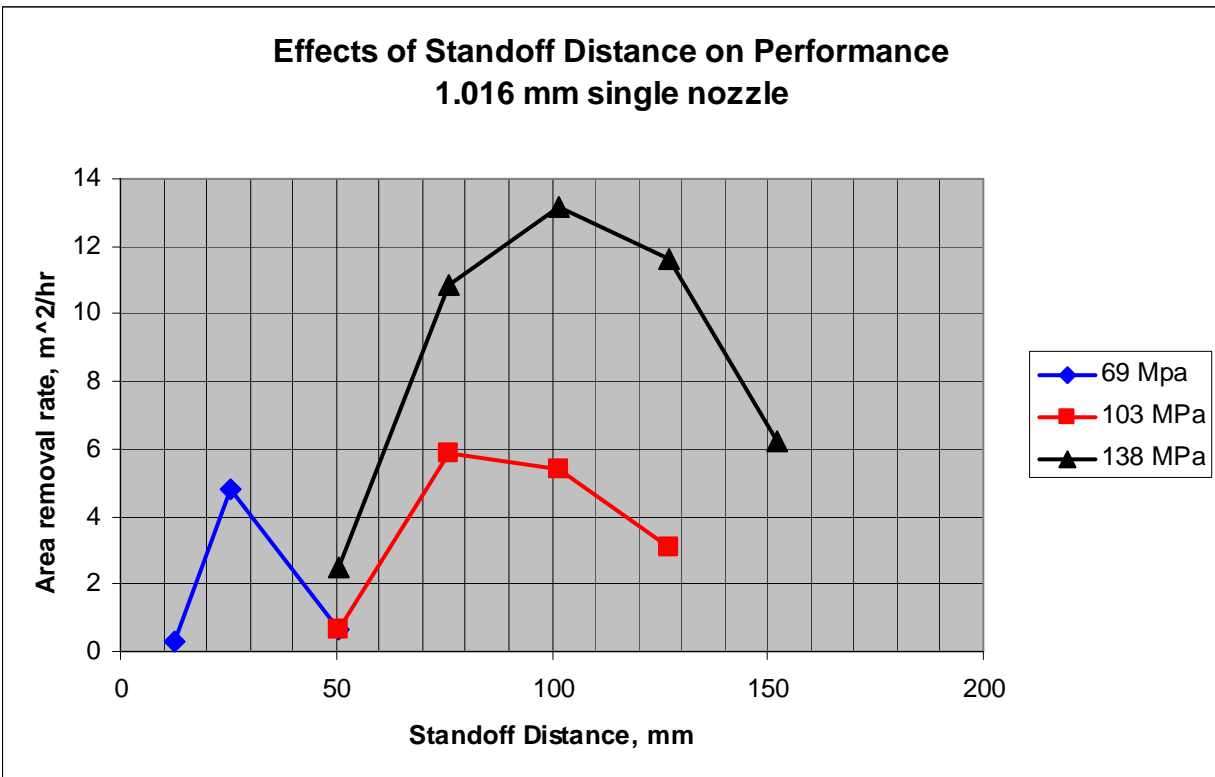
Fig. 2. Plot of removal rate against standoff distance showing the effect of pressure.
