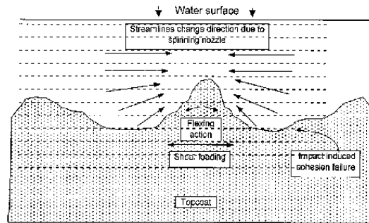
Horizontal flow over the irregular surface, coupled to rapid changes in flow direction as the nozzle spins and moves, induces both high shear loads at the base of any protrusion, and high bending moments.
